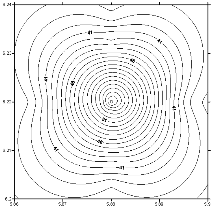
Fig. 5: Mean Temperature Distribution of the area during the Dry Season
