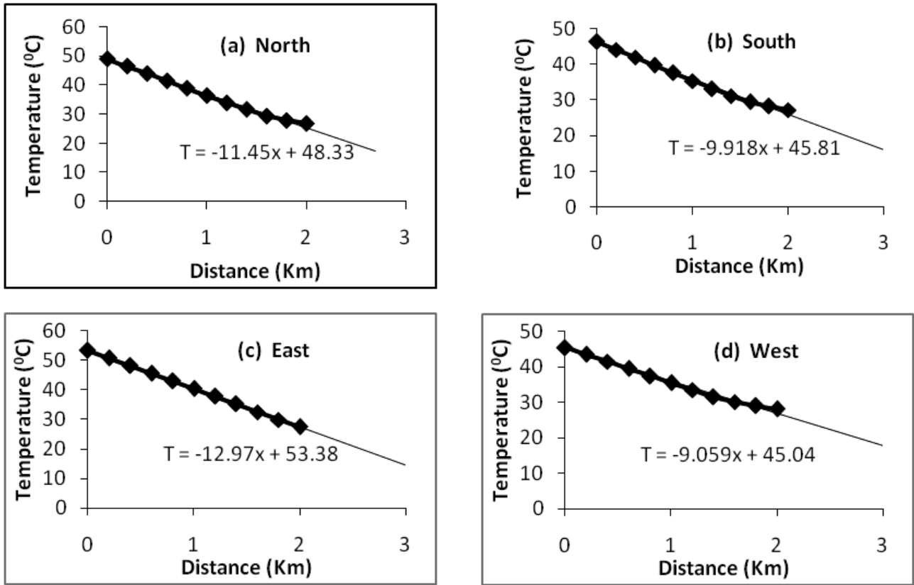
Fig. 2: Variation between mean Temperature and Distance for the raining season.
