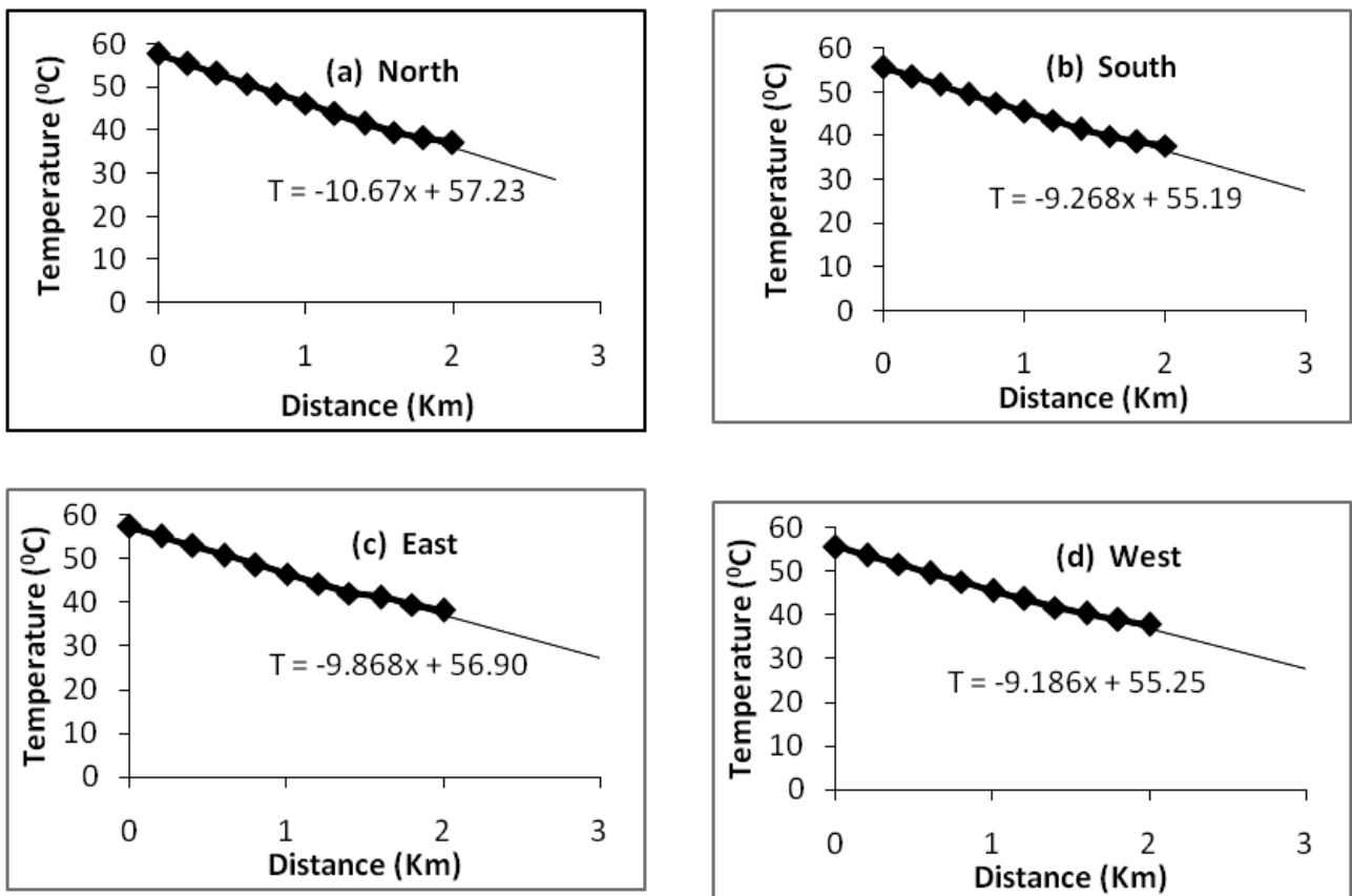
Fig. 3: Variation between mean Temperature and Distance for the dry season.
